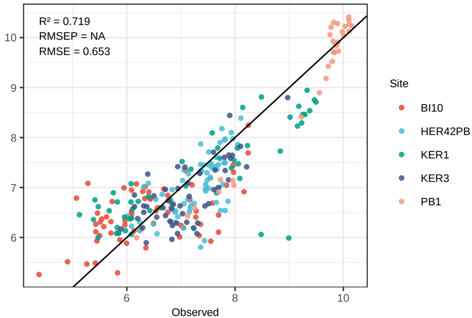
Ti OLS_weighted – Predicted vs Observed (log-space)
